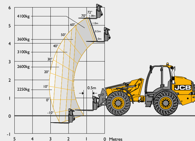
TM420 / TM420S
