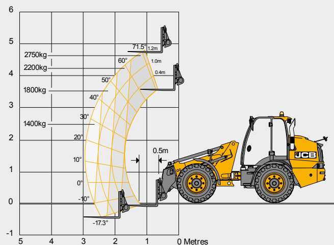
TM280 / TM280S
